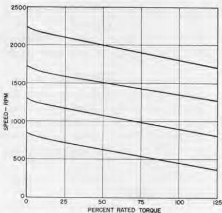
Figure 4. Typical speed-torque curves for the Type 1702-A Variac Speed Control operating a \frac{1}{4} -hp compound motor.
